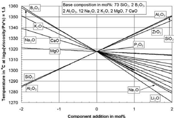
Figure 7. Magnification of Figure 6; spider-graph at \log(\eta/(Pa\cdot s))=1.5
