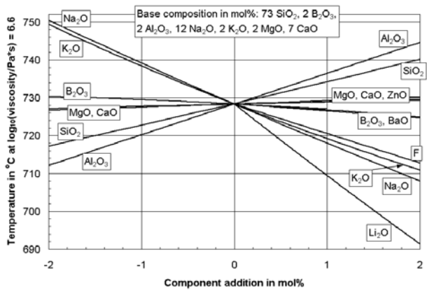
Figure 10. Magnification of Figure 9; spider-graph at \log(\eta/(Pa\cdot s))=6.6 (~Littleton Softening Point)
