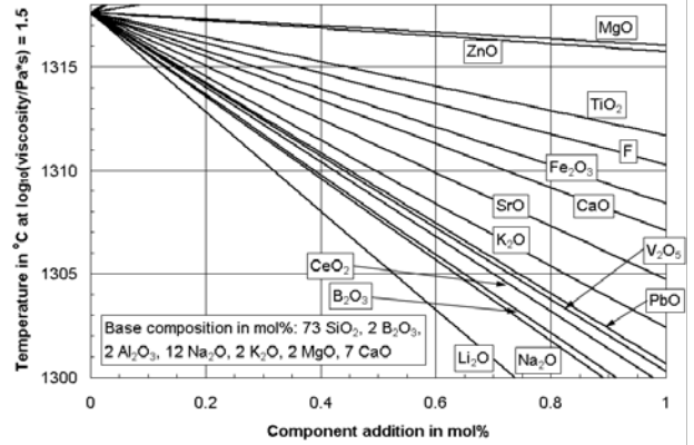
Figure 8. Magnification of Figure 7, spider-graph at \log(\eta/(Pa\cdot s))=1.5 ; polyvalent oxidation states other than those shown in the figure must be converted to the given oxides on a molar basis. The 95% confidence interval of the model mean in Figure 8 is 3–8°C, depending on the glass composition
