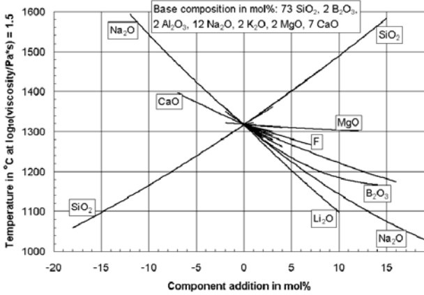
Figure 6. Spider-graph for the given specific base composition using the model at \log(\eta/(Pa\cdot s))=1.5 ; the spider-graph is different for other base compositions. For any component addition the ratios of all the remaining components remain constant
