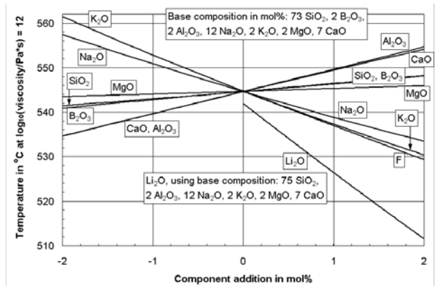
Figure 12. Magnification of Figure 11, spider-graph at \log(\eta/(Pa\cdot s))=12.0 ; to demonstrate the influence of Li 2 O this graph is based on a slightly different base composition to previous figures because of the limits of validity of the model
