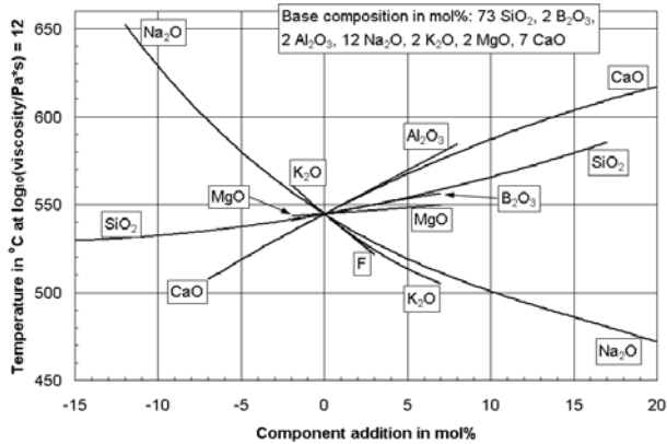
Figure 11. Spider-graph for the given specific base composition using the model at \log(\eta/(Pa\cdot s))=12.0 ; The spider-graph is different for other base compositions. For any component addition the ratios of all the remaining components remain constant
